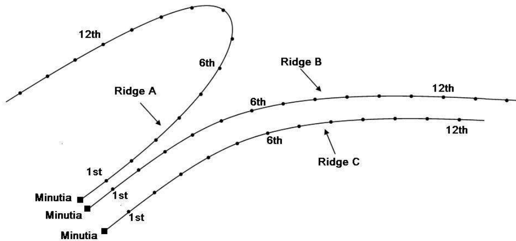
Fig. 6. Effectiveness of ridge point selection scheme: ridges B and C are genuine ridges in different impressions. Through proper transformation, B and C will simultaneously have overlapping minutiae, overlapping 6^{th} RRPs and overlapping 12^{th} RRPs. However, ridges A and B (two different ridges) could not have overlapping minutiae and overlapping RRPs at the same time, although they might occasionally have overlapping RRPs or overlapping minutiae separately.
