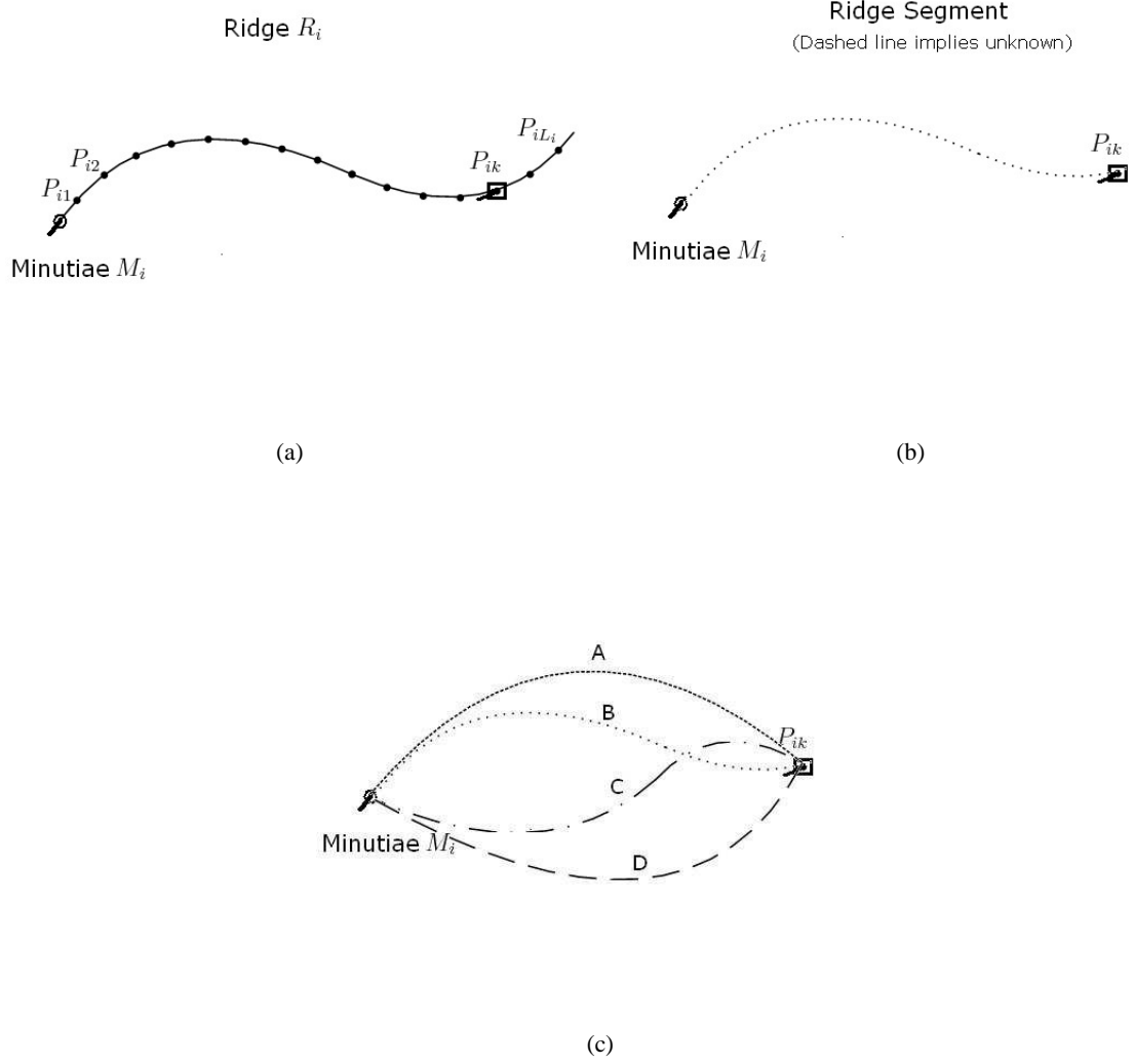
Fig. 8. Implication from minutiae and the k^{th} ridge points to ridge segment. (a) a ridge with minutia and ridge points, (b) the k^{th} ridge point is selected as RRP, (c) four possible candidate shapes of the ridge segment with fixed segment length kd and fixed positions of both the two end points.
