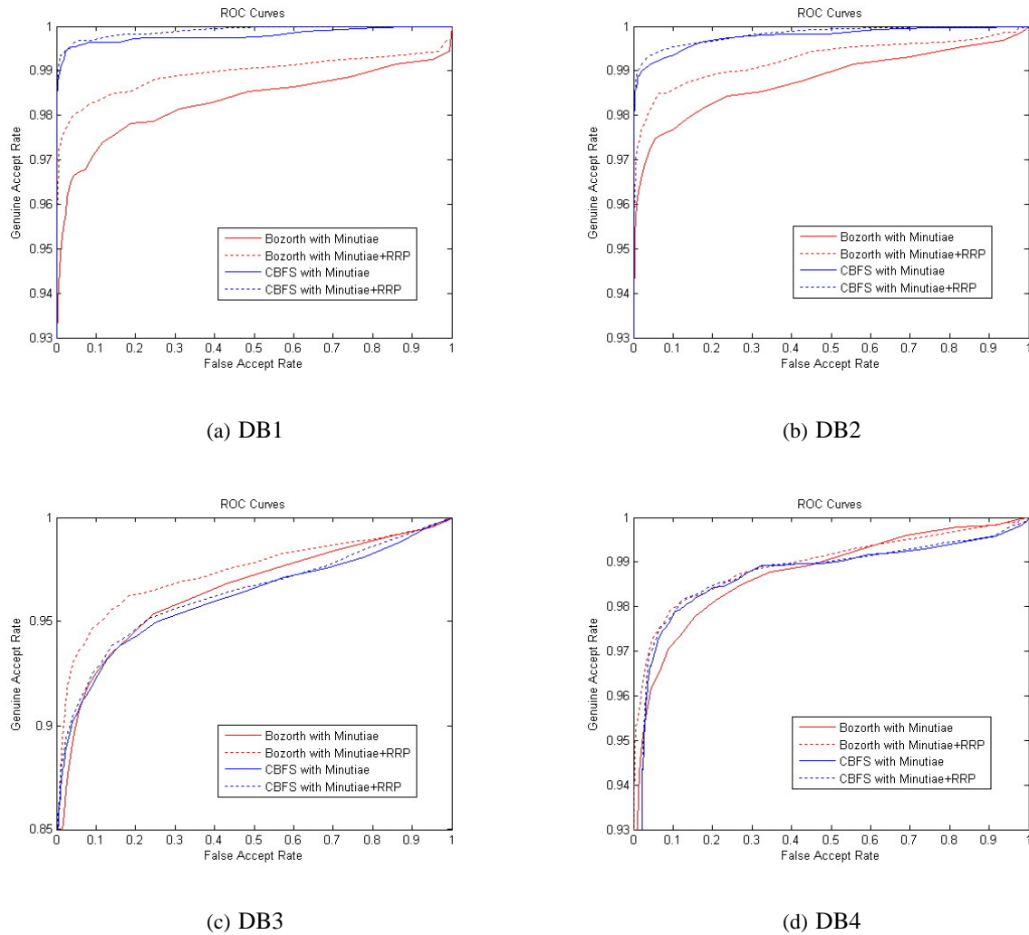
Fig. 10. ROCs of full fingerprint matching with the four databases DB1-DB4 in FVC2002. The four curves correspond to pairwise matching (Bozorth) and k minutiae matching (CBFS) with and without RRP. In each case the ROC of minutiae+RRPs is fully above the ROC of minutiae only.
