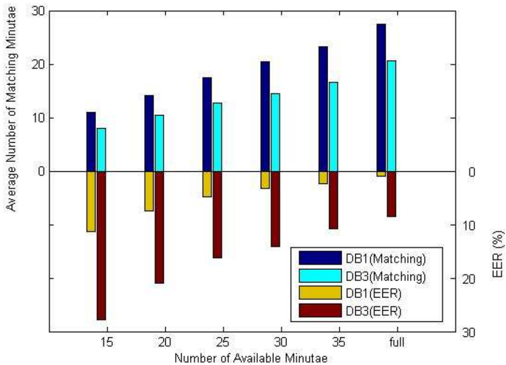
Fig. 4. Effect of number of input minutiae on: (i) number of minutiae that match with the genuine full print (top half of chart), and (ii) equal error rate (EER) (bottom half of chart). As the number of minutiae increases, the number of matched minutiae increases and the EER decreases. The partial images were generated from images in FVC2002– data sets DB1 and DB3. The average number of minutiae of full fingerprints in DB1 and DB3, as detected by MINDTCT [1], were 43 and 53 respectively.
