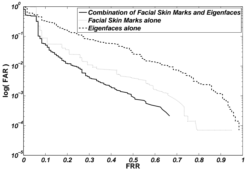
Figure 2.12. ROC curves for three person identification systems: the system utilizes Eigenfaces alone as biometric trait shown in dashed curve, the system utilizes facial skin mark alone as biometric trait shown in dotted curve, and the system utilizes combined biometrics of Eigenfaces and facial skin mark shown in solid curve. The FAR axis was log-scaled in order to better show the performance of these algorithms for small FAR values.
