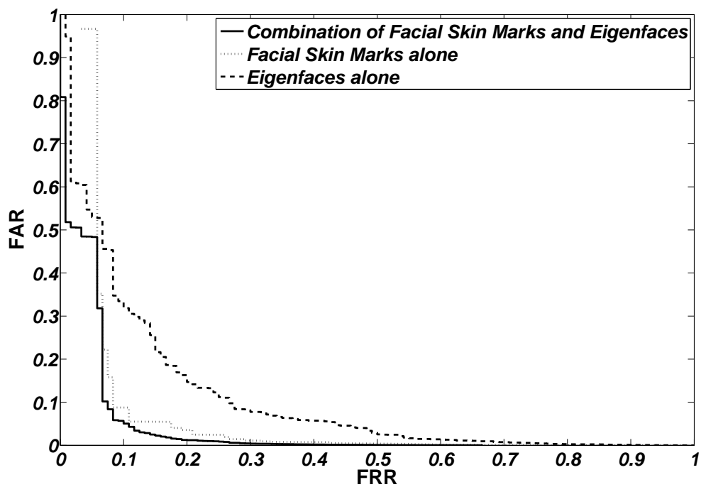
Figure 2.11. ROC curves for three person identification systems: the system utilizes Eigenfaces alone as biometric trait shown in dashed curve, the system utilizes facial skin mark alone as biometric trait shown in dotted curve, and the system utilizes combined biometrics of Eigenfaces and facial skin mark shown in solid curve.
