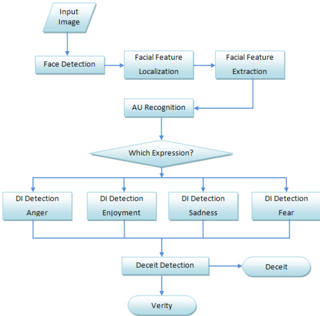
Figure 3.4. The framework of deceit detection system based on reliable facial expressions through DI detections.
