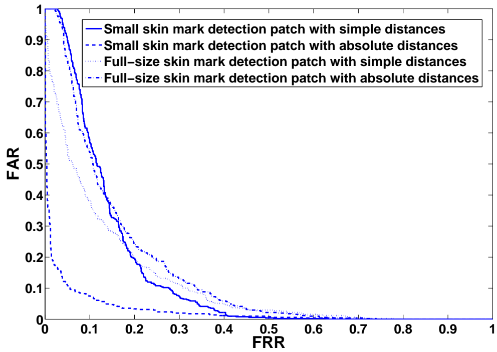
Figure 2.7. ROC curves for different facial skin mark detection scenarios. System and parameter settings details are shown in Table 2.3.
