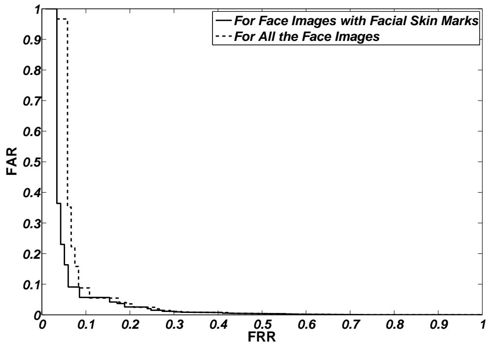
Figure 2.10. ROC curves for person identification system based on biometric trait of facial skin marks alone. The solid curve shows the ROC curve for system testing on facial images with enough facial skin marks shown, while the dotted curve shows the ROC curve for system testing on all the available facial images in the facial skin mark dataset.
