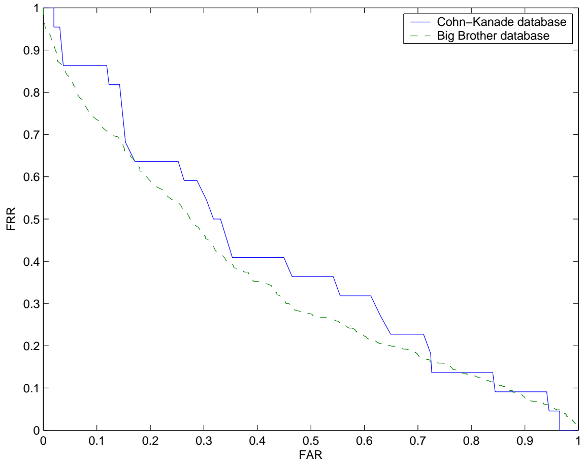
Figure 4.4. ROC performance curves for face expression biometrics on two databases.
