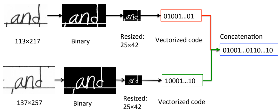
Fig. 4: Vectorization for image-based verification.
