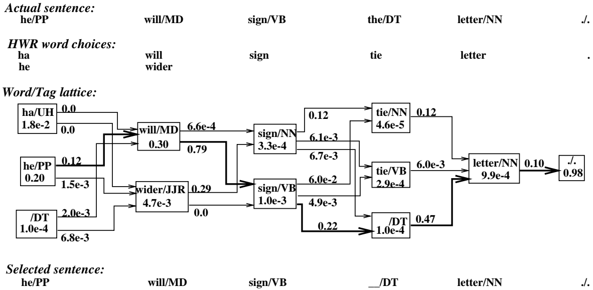
Figure 4: Sample Word:Tag Lattice For Analysis of WR choices
