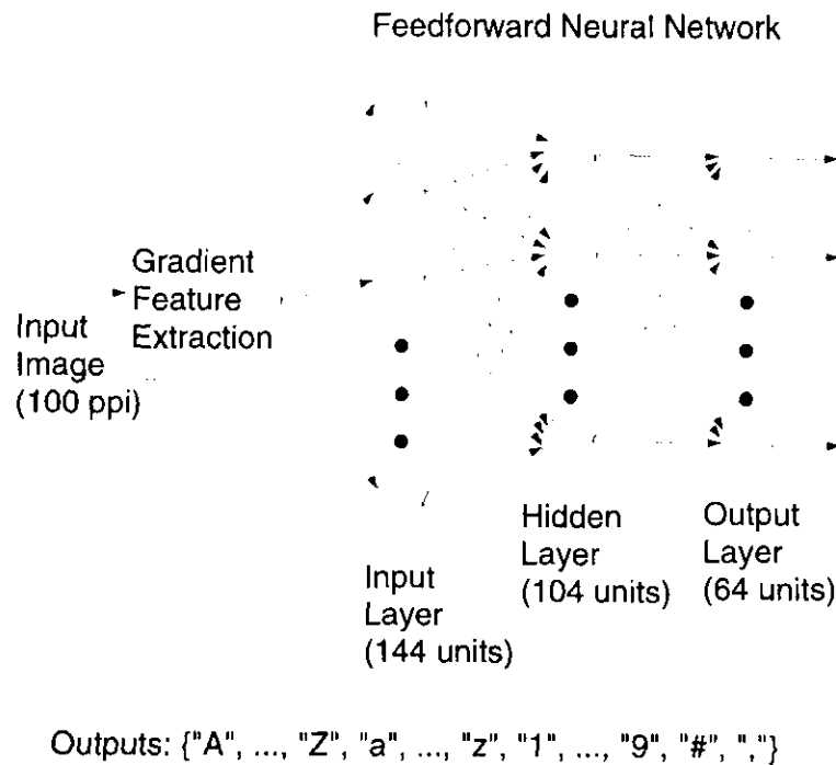
Figure 5.4: A method of performing character recognition.
