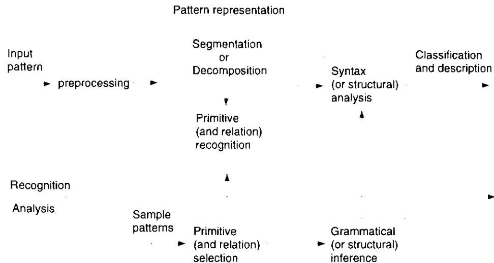
Figure 2.1: Block diagram of a syntactic pattern recognition system. (From Fu, 1982.)
