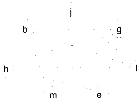
Connection graph of L 2
