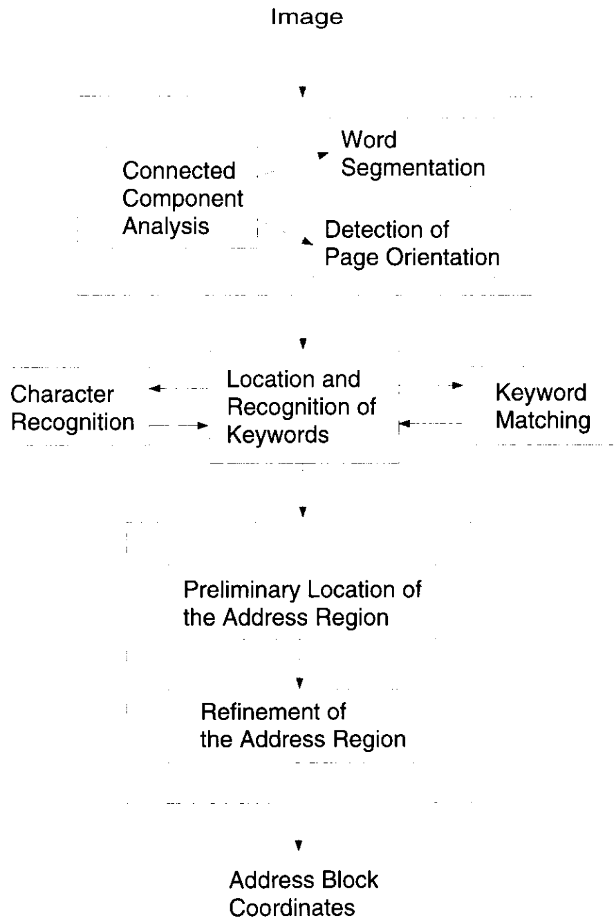
Figure 6.5: Fax address block location system design.
