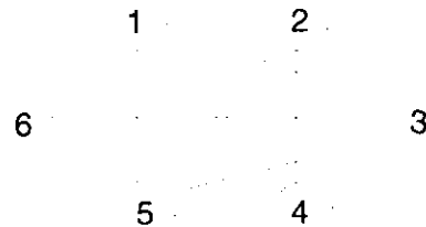
Connection graph of U1
