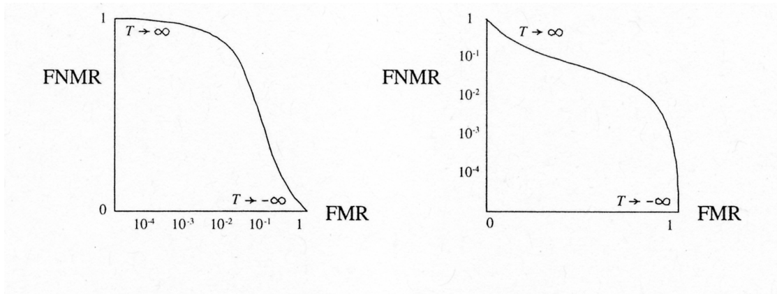
Figure 5.5: The ROC with one probability scale in logarithmic form; on the left the FMR is expressed in logarithmic form, on the right the FNMR is in logarithmic form.
