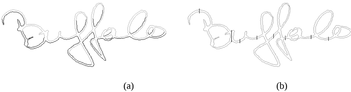
Fig. 3. (a) Splitting a contour to upper and lower parts. The upper contour is shown in dotted lines and the lower contour is shown in bold lines, (b) character segmentation points are potentially found at the central part of ligatures; a segmentation point is found between 'B' and 'u' by heuristic rules that cut at points where the maxima of the upper contour is in close proximity to the minima of a lower contour.
