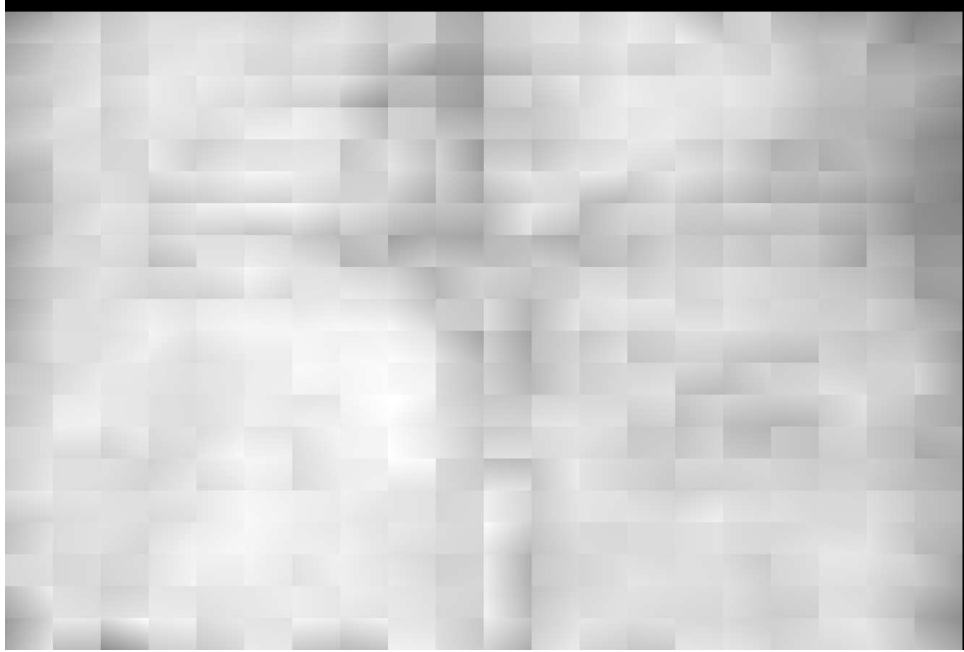
Figure 4: Piece-wise linear approximation of the background for the image in Figure 3.
