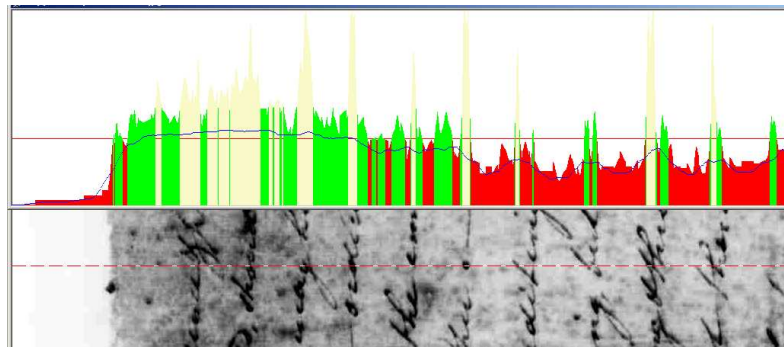
Figure 5: Scanline histogram and background approximation. The histogram of black pixel intensity along a selected scanline is shown above the grey-scale document. The horizontal line is the calculated average level. The curve is the approximation of the background.
