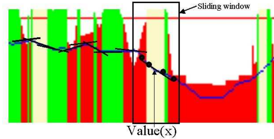
Figure 6: Background approximation along a scanline: Step 1: Filter foreground pixels as before Step 2: For each scan line derive new intensity values. Use a sliding window positioned at the point x . Use sliding window for local line fitting to derive \text{value}(x) from the existing background pixel values. The approximated curve is an envelope of the line segments.
