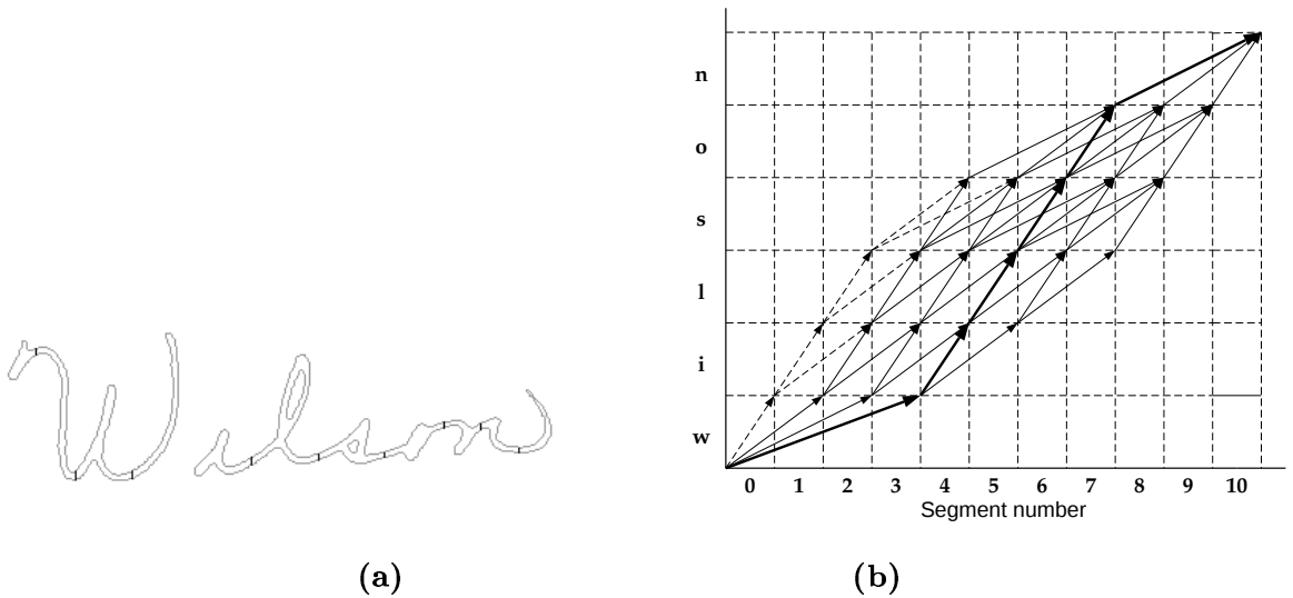
Figure 13: (a) Image features based dissection of a word image, (b) dynamic matching of the segments (intermediate entities) with the lexicon word WILSON.
