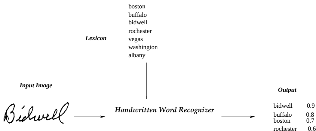
Figure 1: I/O behavior of off-line HWR. Input is the word image and a lexicon of possible choices. Output is the lexicon sorted by some confidence measure.
