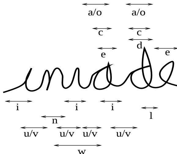
Figure 14: Looking for instances of each character in a lexicon word (INVADE in this example) in the word image.
