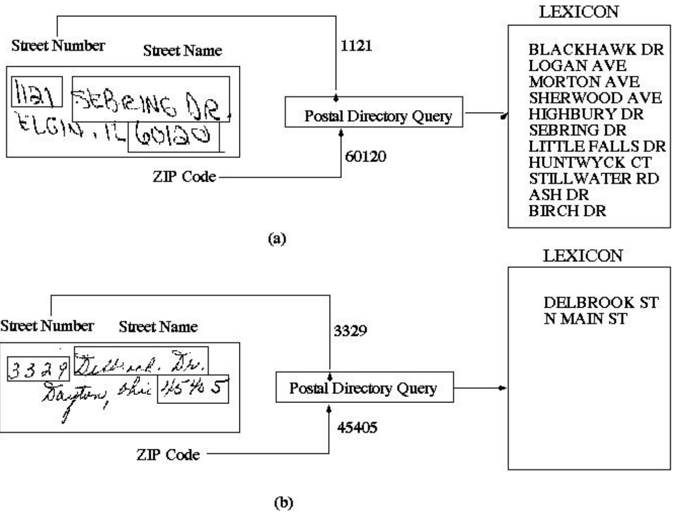
Figure 4: Lexicon is dynamically created using the ZIP Code and the street number. Note that the street name images are matched with different lexicons generated. (a) In ZIP Code 60120 there are 11 streets which have the street number 1121. (b) In ZIP Code 45405 there are 2 streets with the street number 3329.
