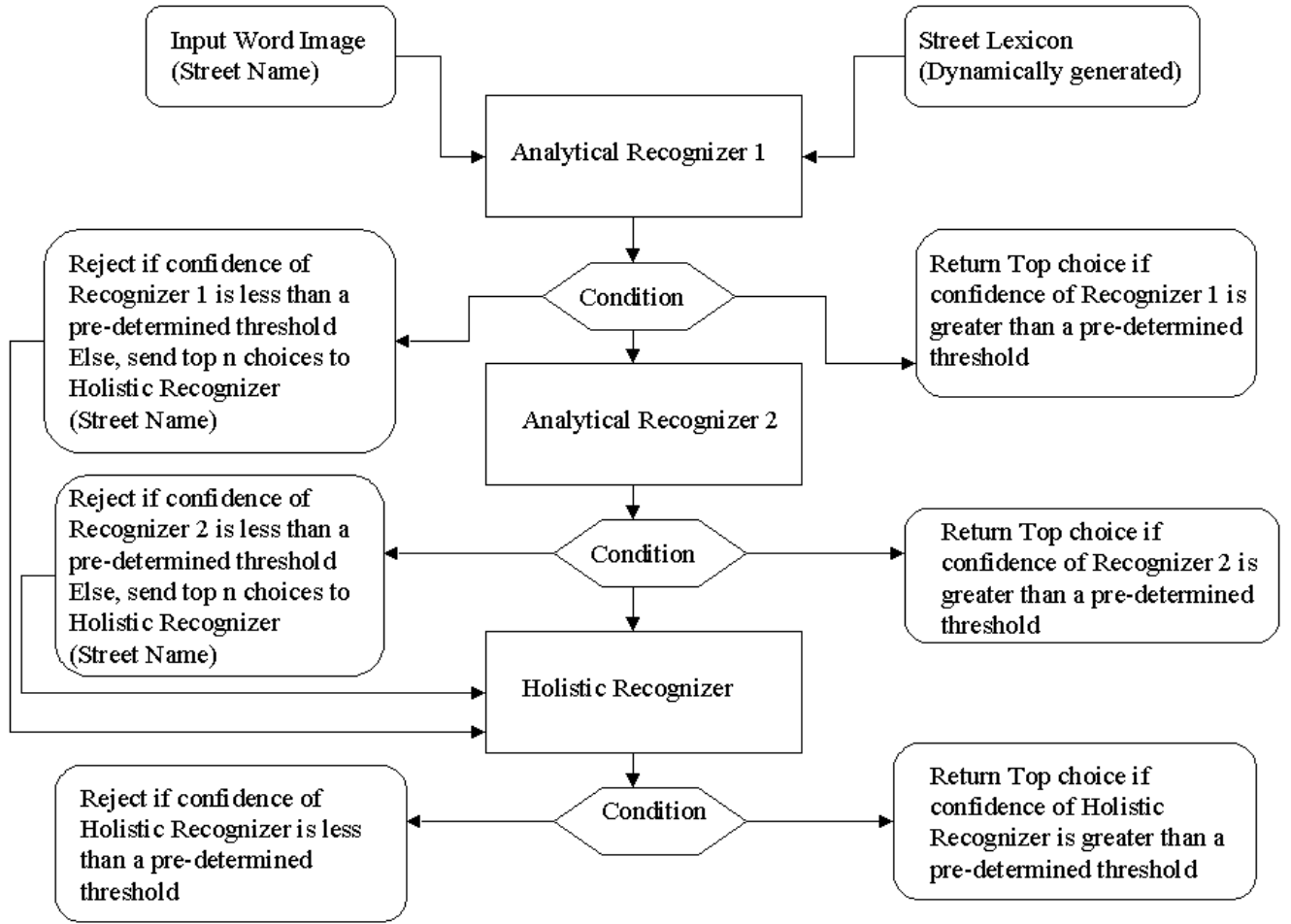
Figure 8: Combination of three word recognizers, two analytical and a holistic in the context of handwritten address interpretation. The holistic recognizer serves as a ‘tie-breaker’ between the top choices of the two analytical recognizers.
