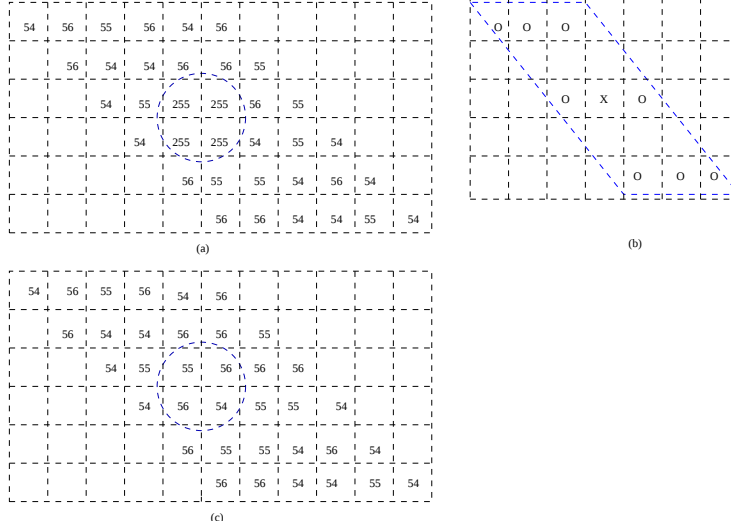
Fig. 5. Filling out the hole in fingerprint image. (a)image with one hole, (b)Median template with the same direction as the ridge, (c) filtered image
