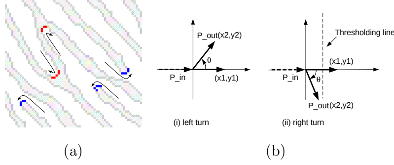
Fig. 6. (a) Minutia location on chaincode. (b) The distance between the thresholding line and the y -axis gives a threshold for determining a significant turn.
