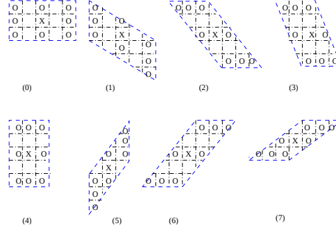
Fig. 2. Eight directional templates, following orientation definitions
