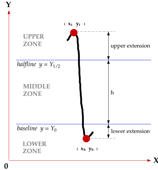
Figure 7: Upper and lower extensions of a stroke: The coordinates of the limiting contour extrema may be used to compute the upper and lower extensions of the stroke in the offline case.
