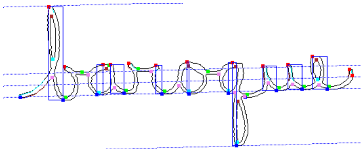
Figure 6: Evidence from upper and lower chords is combined using knowledge of valid spatial configurations of chords to detect downstrokes, indicated by bounding rectangles.
