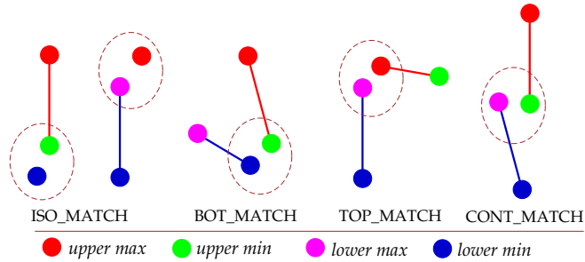
Figure 4: Basic categories of chord configurations that define downstrokes
