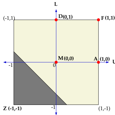
Figure 8: The U-L representation space: The dark region corresponds to the strokes rendered invalid by the use of a threshold \theta on the normalized extent (shown for \theta = 0.25 ).
