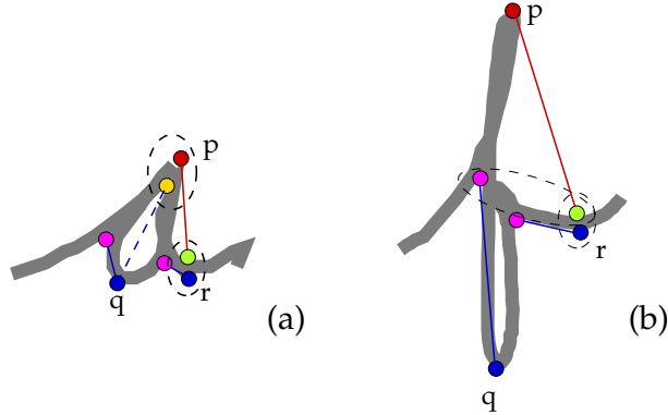
Figure 5: Spatial chord configurations in two sample cursive characters. In (a), the upper maximum p may be matched with lower minimum q using the TOP_MATCH criterion, by invoking the auxiliary chord of q . p may be matched with lower minimum r using the BOT_MATCH criterion. In (b), CONT_MATCH may be used to match upper maximum p with lower minimum q . Following the CONT_MATCH, p is prevented from matching subsequent lower minima such as r .
