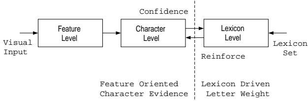
Figure 2: Lexicon-Adaptation Recognition
