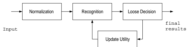
Figure 1: recursive recognition
