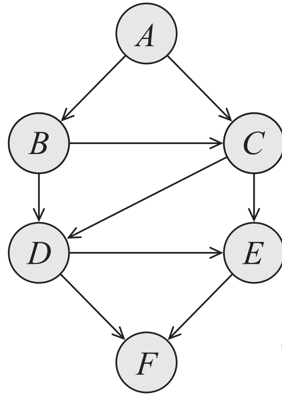
Minimal I-map BN
