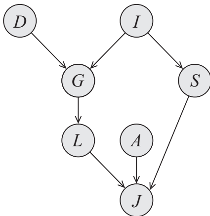
Bayesian Network G
