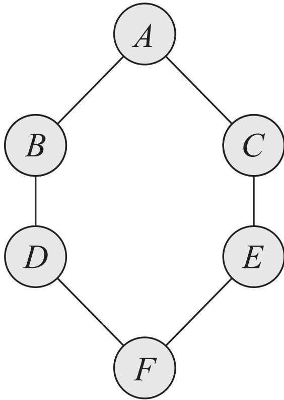
MN with a loop
