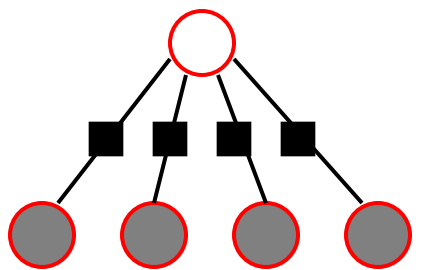
Logistic Regression
