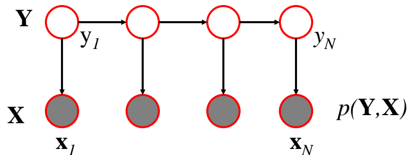
Hidden Markov Model
