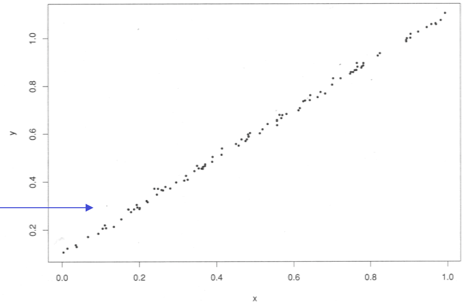
Figure 2.2 A simple nonlinear relationship between variable V_1 and subsequent figures V_1 and V_2 are on the X and Y axes respectively
