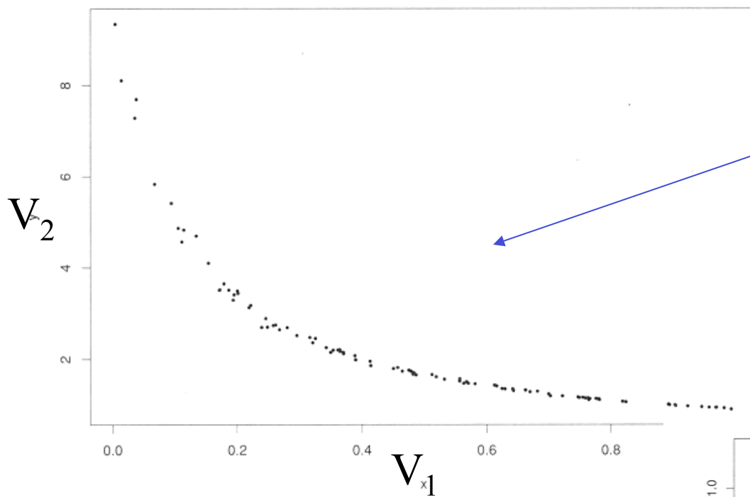
Figure 2.2 A simple nonlinear relationship between variable V_1 and subsequent figures V_1 and V_2 are on the X and Y axes respectively
