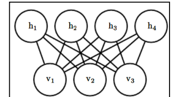
An RBM
