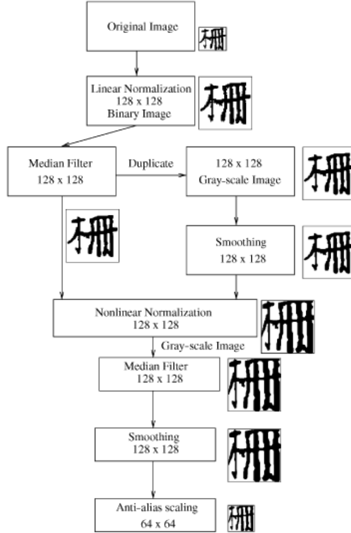
Figure 10: Normalization process from [64]. The transformed image is shown beside each box.
