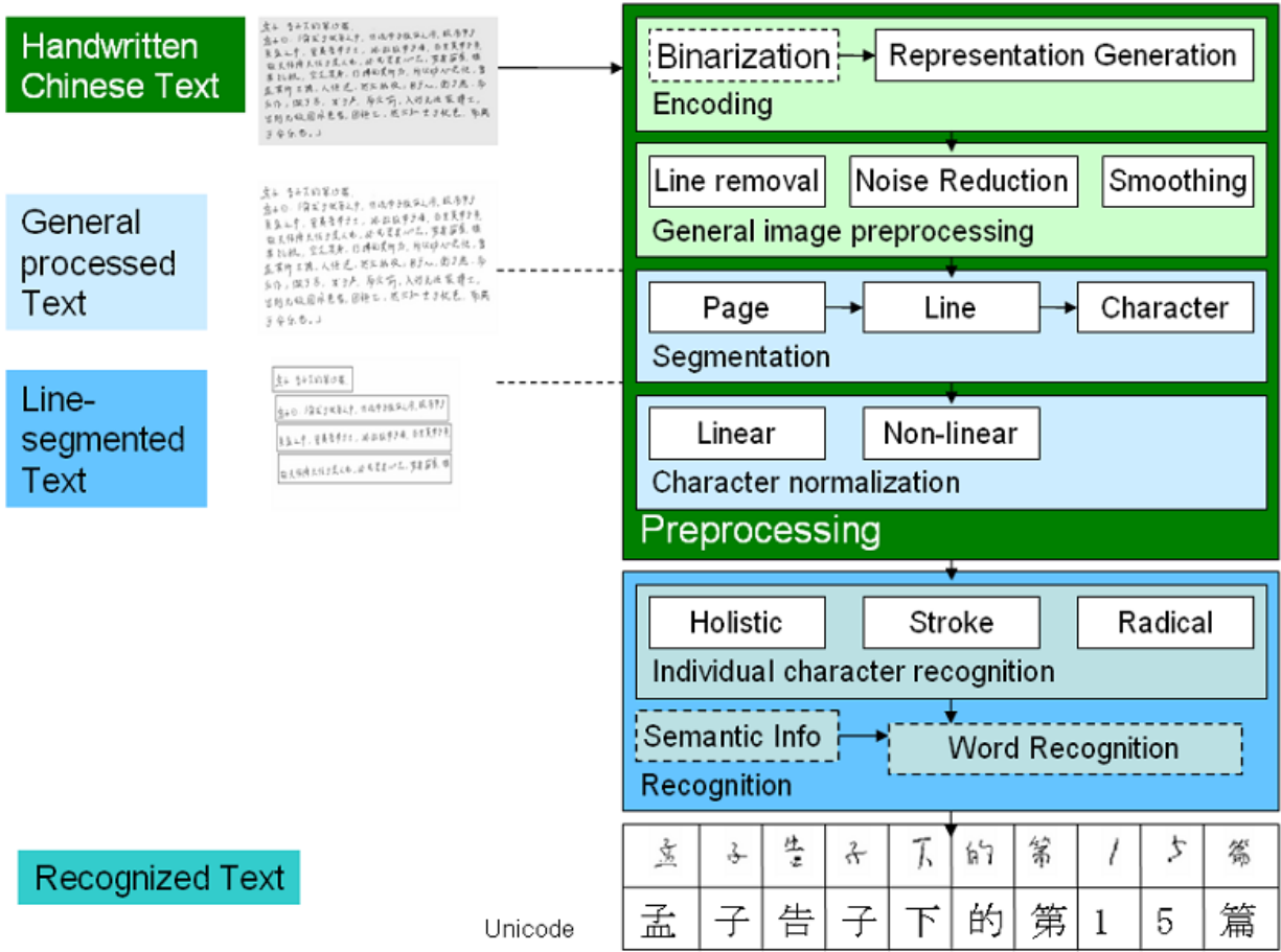
Figure 4: Process of Chinese Handwriting Recognition
