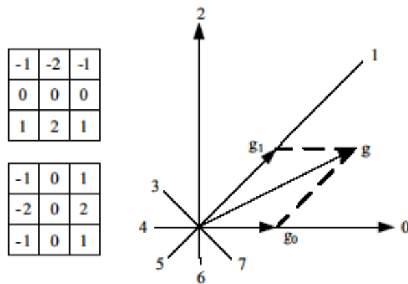
Figure 13: Gradient feature extraction using Sobel operators and gradient vector decomposition (eight directions for illustration)
