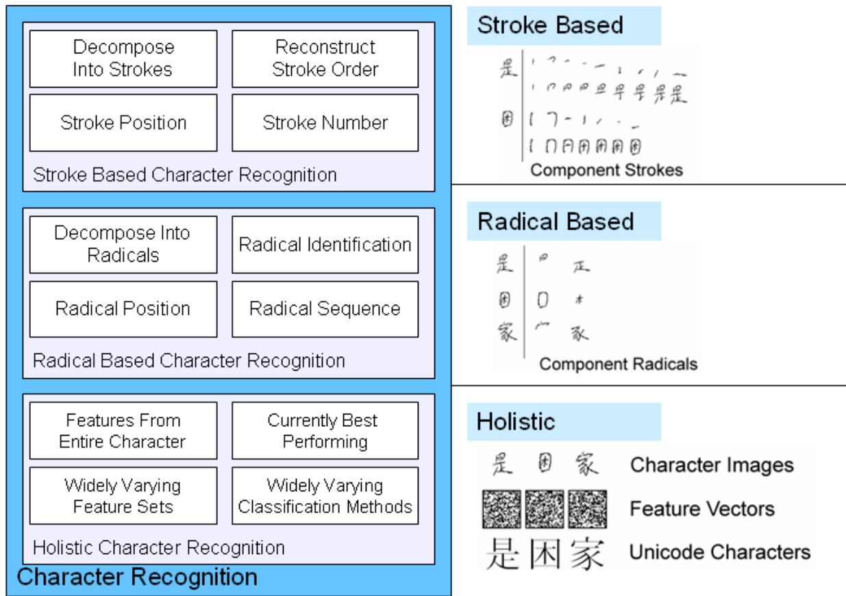
Figure 12: Character recognition
