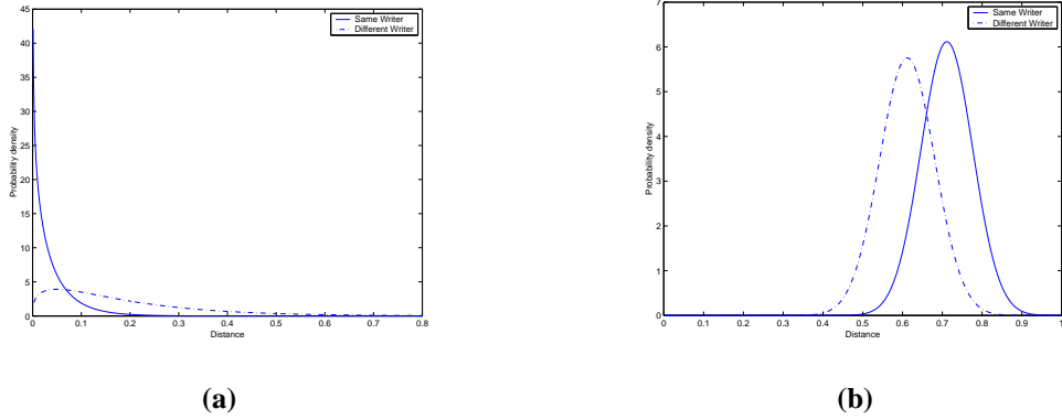
Figure 3. Parametric pdfs for: (a) entropy (gamma distributions) and (b) numeral 3 (Gaussians).
