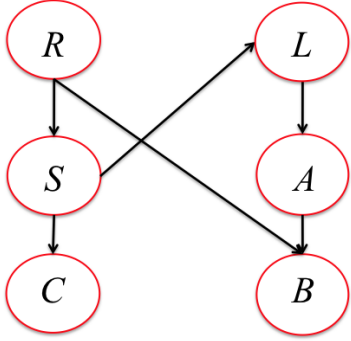
Figure 2. Bayesian network BN_{th} : this graph together with CPDs in Section III defines the probability distribution of the characteristics of th .
