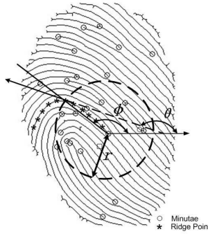
Fig. 4. Representation of ridge points in polar coordinates.
