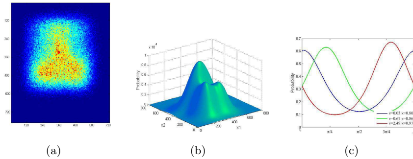
Fig. 3. Model for minutiae distribution: (a) Distribution of minutiae location from NIST special database, (b) Three-dimensional plot of mixture Gaussian model for minutiae location with three components, (c) von Mises distributions of minutiae orientation for each of the three components, where the green curve corresponds to the upper cluster, blue the lower left cluster and red the lower right cluster.
