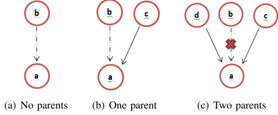
Figure 1. Heuristics of determining Structure in Algorithm BNSL
