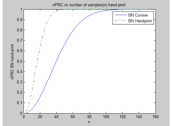
Figure 3. n PRC vs n for cursive and handprint datasets. Cursive dataset is more individualistic
