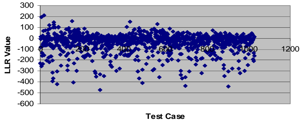
Different Writer Distribution
